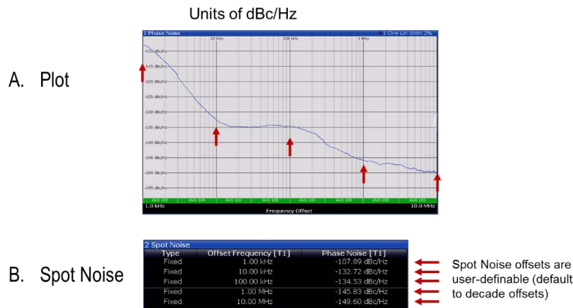
Fig. 2-4: Quantifying phase noise.
