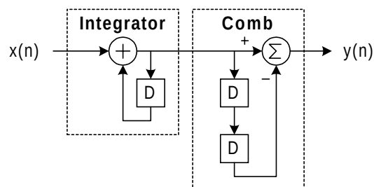
Figure 9.28. Double Delay CIC Decimator
