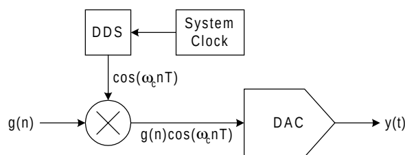
Figure 9.10. DDS Modulator
