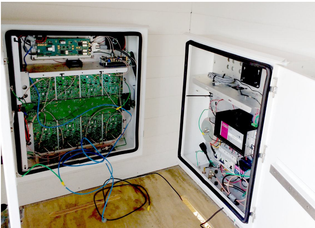
High frequency radar scatterometer installed on behalf of Woods Hole Oceanographic Institution (April 2018). On the left, receiver box, signal generator and analogue-digital converter in the upper compartment; reception cards and bandpass filters in the lower compartment. On the right, power supply box with circuit breakers, relays, power supplies, isolation transformer in the lower compartment; mounting plate for the control computer in the upper compartment.
