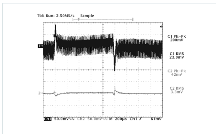
Figure 12.15 — V48C5C100B and \mu RAM; Input and output dynamic response no added C_{TRAN} ; 23% of 20A rating load step of 4.5A (10 – 14.5A); R_{HR} = 31k\Omega (Configured as in Figures 12.1a and 12.1b)
