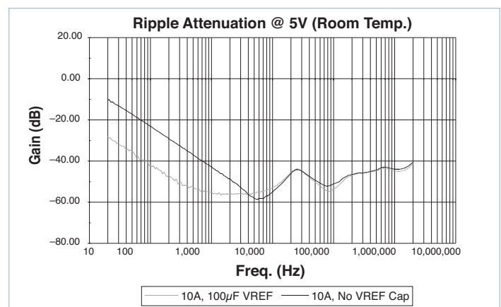
Figure 12.3b — The small signal attenuation performance as measured on a network analyzer with a typical module at 5V and 10A. The low frequency attenuation can be enhanced by connecting a 100 \mu F capacitor, C_{HR} , to the VREF pin as shown in Figures 12.1 and 12.2
