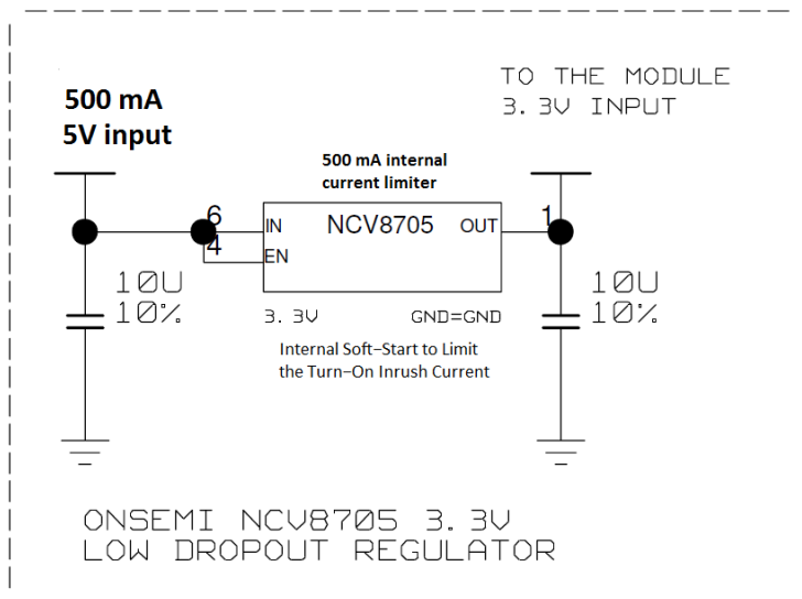
Figure 30: ZED-F9T power supply
