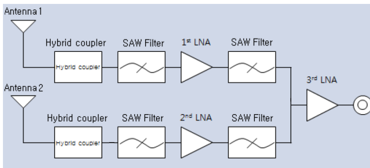
Figure 32: u-blox low cost dual-band antenna internal structure
