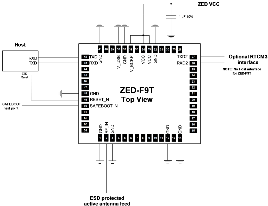
Figure 31: Minimal ZED-F9T design
