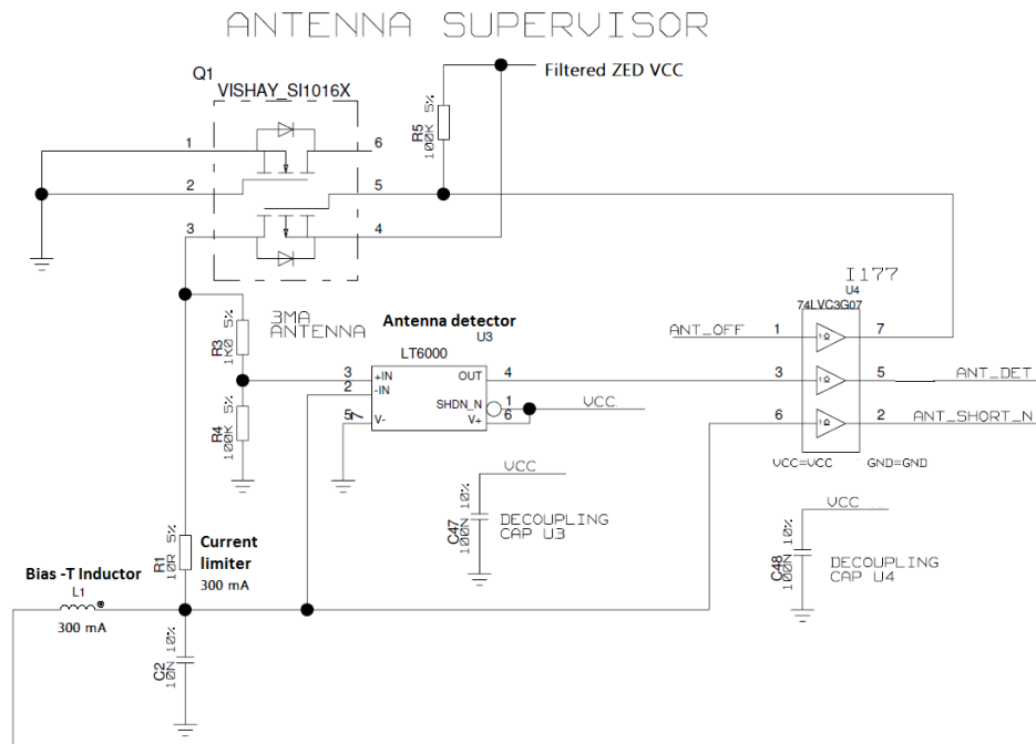
Figure 17: ZED-F9T antenna supervisor
