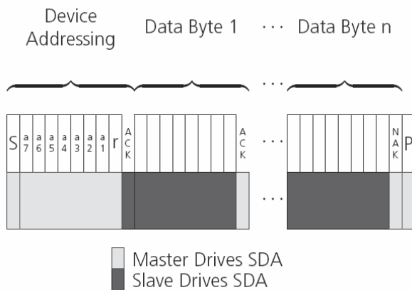
Figure 13: I2C current address read access
