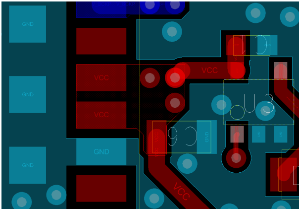
Figure 43: VCC pads
