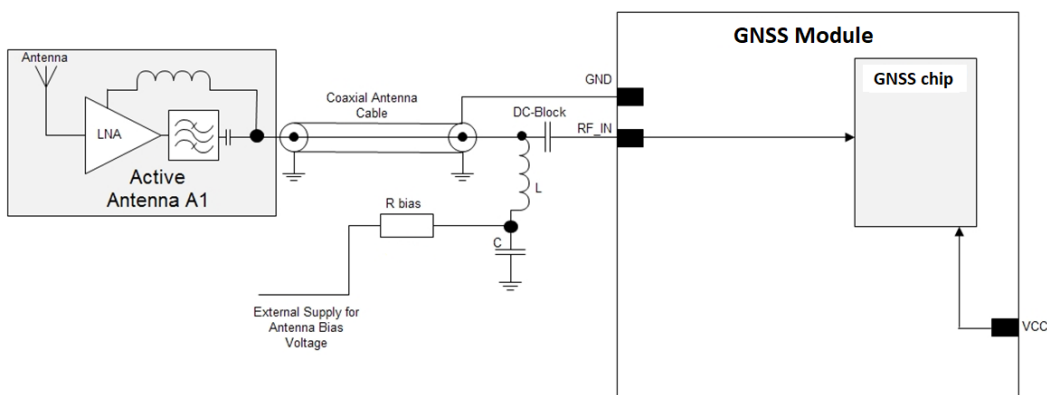
Figure 36: ZED-F9T external voltage antenna bias
