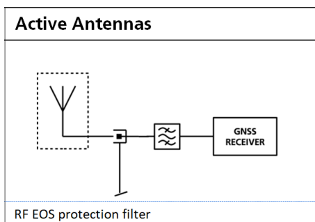
Figure 38: Active antenna EOS protection
