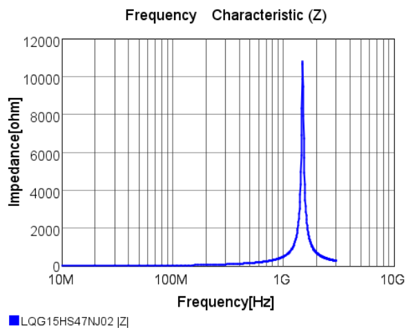
Figure 33: ZED-F9T antenna bias inductor impedance
