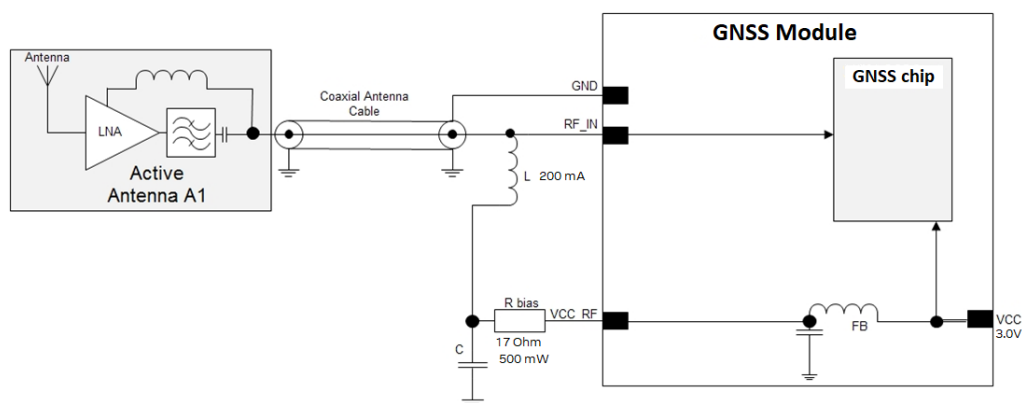
Figure 35: ZED-F9T VCC_RF antenna bias
