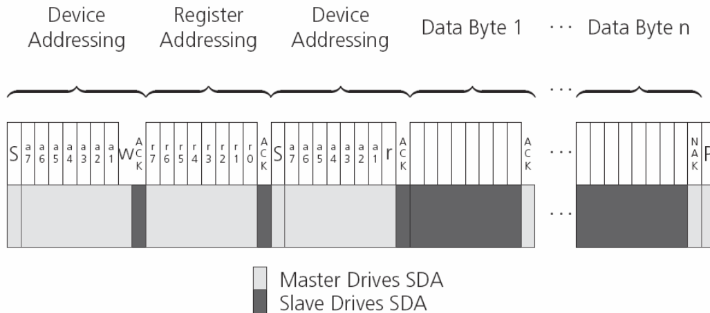
Figure 12: I2C random read access
