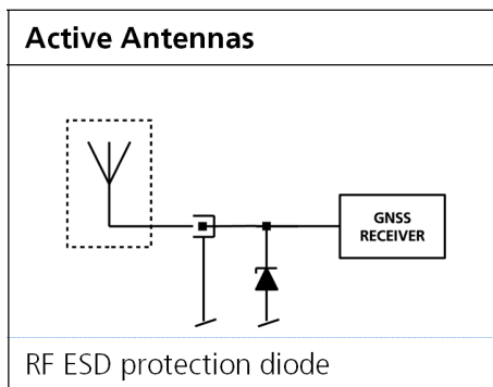
Figure 37: RF ESD precautions
