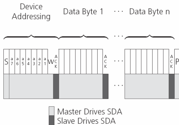
Figure 14: I2C write access
