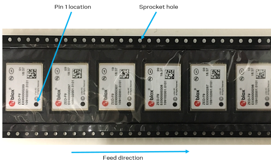
Figure 45: Orientation of ZED-F9T on the tape
