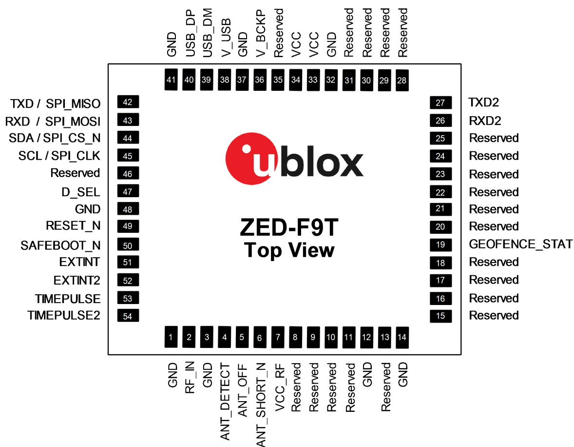
Figure 29: ZED-F9T pin assignment
