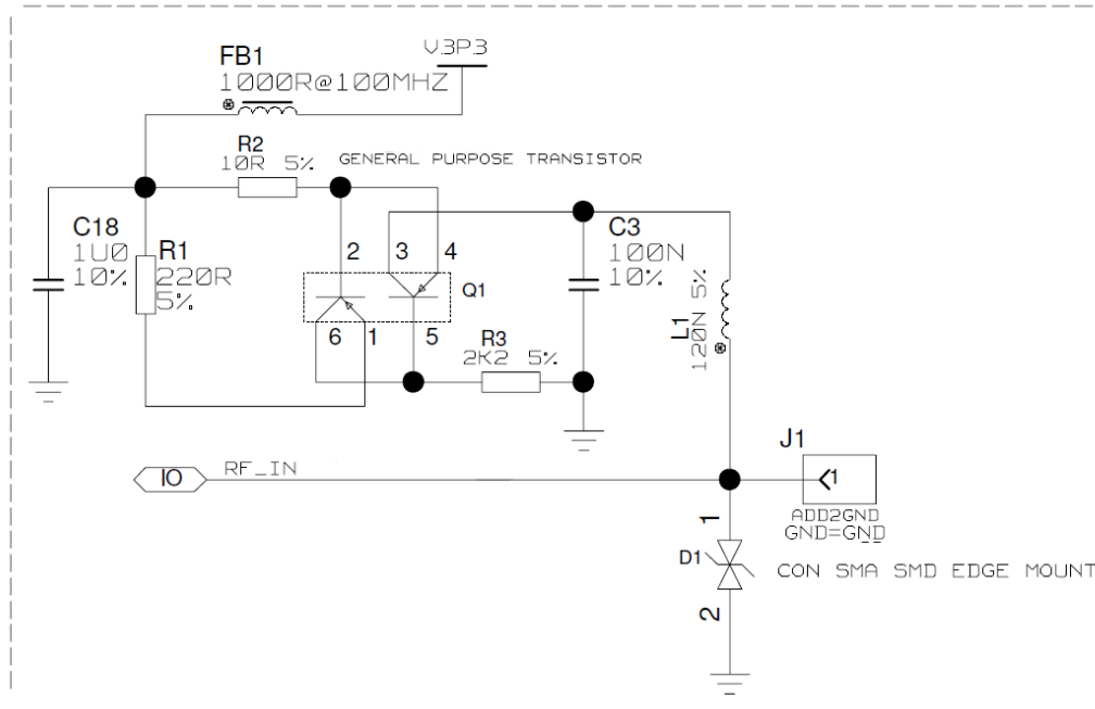
Figure 34: ZED-F9T reference design for antenna bias
