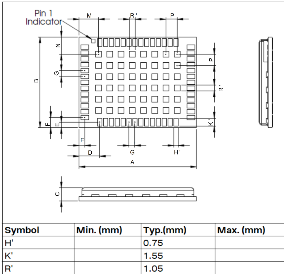
Figure 40: ZED-F9T suggested paste mask
