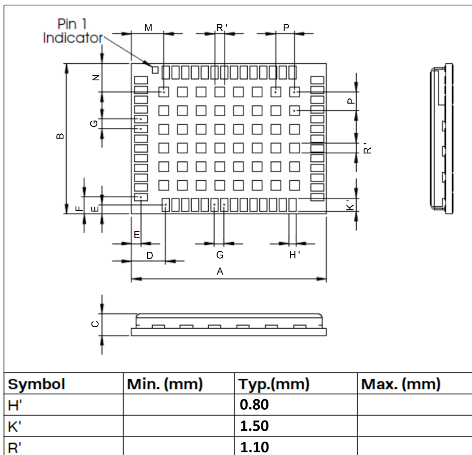
Figure 39: ZED-F9T suggested footprint (i.e. copper mask)
