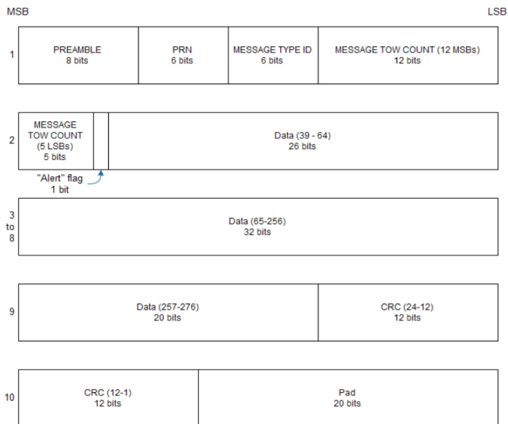
Figure 24: GPS L5 subframe words
