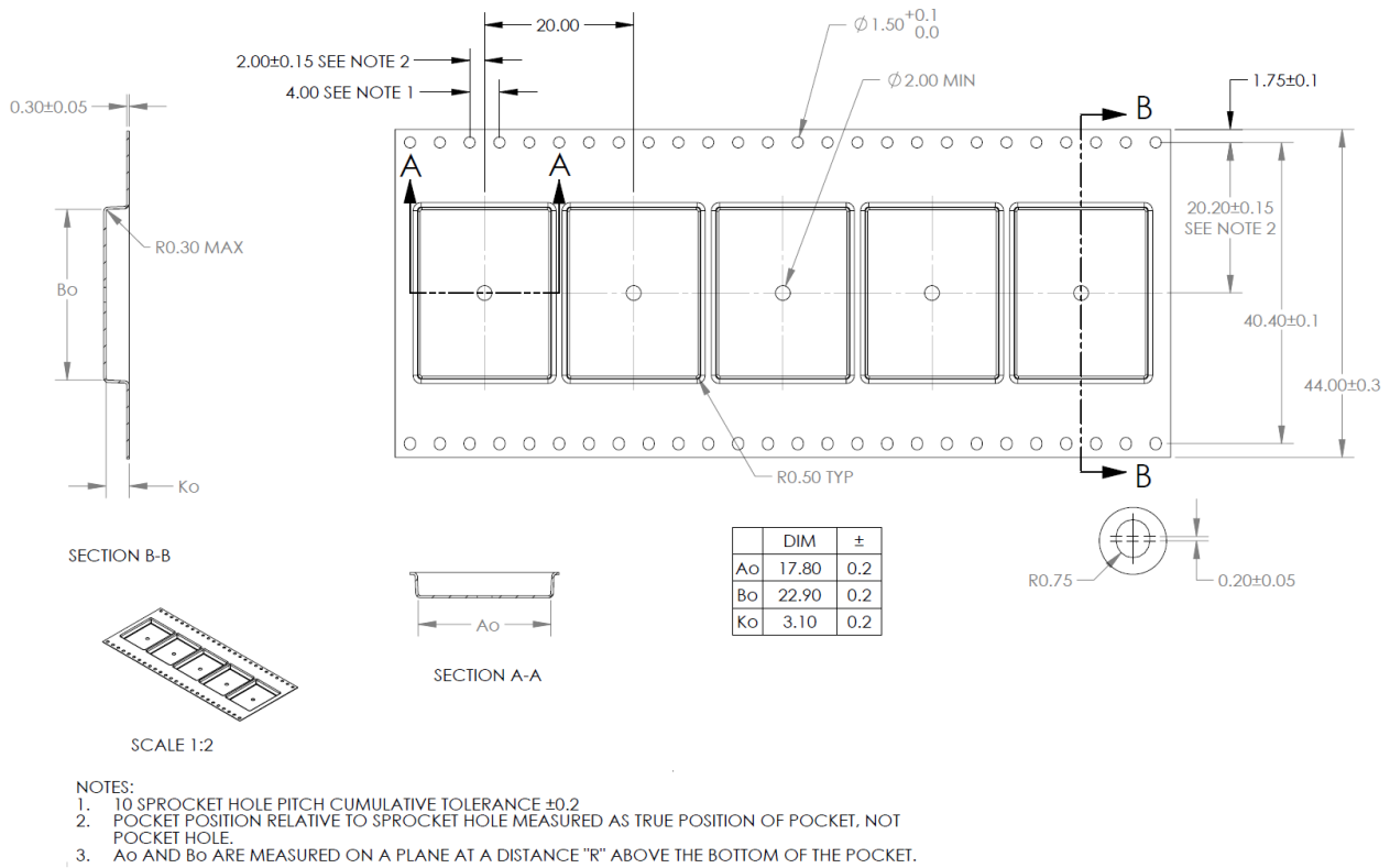
Figure 46: ZED-F9T tape dimensions (mm)
