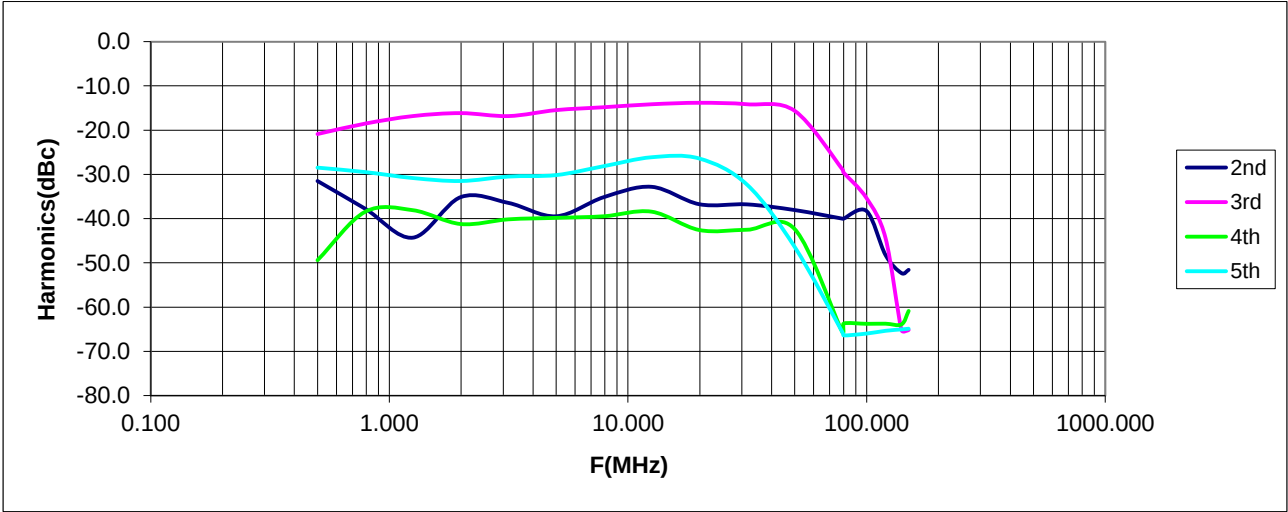
Harmonics Measured @ Pout = P1dB spec.
