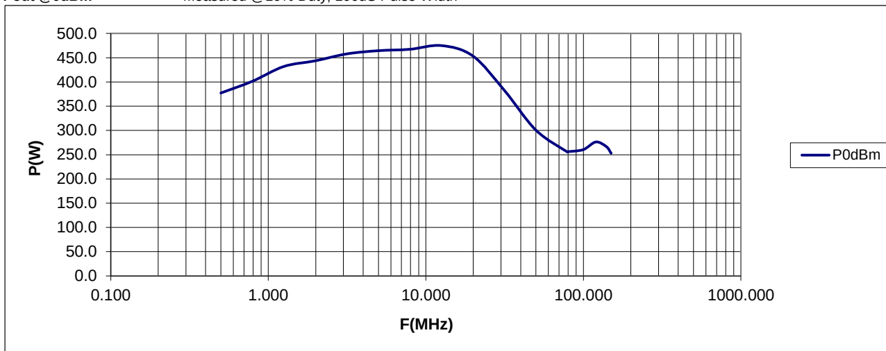
P1dB Measured @10% Duty, 100uS Pulse Width
