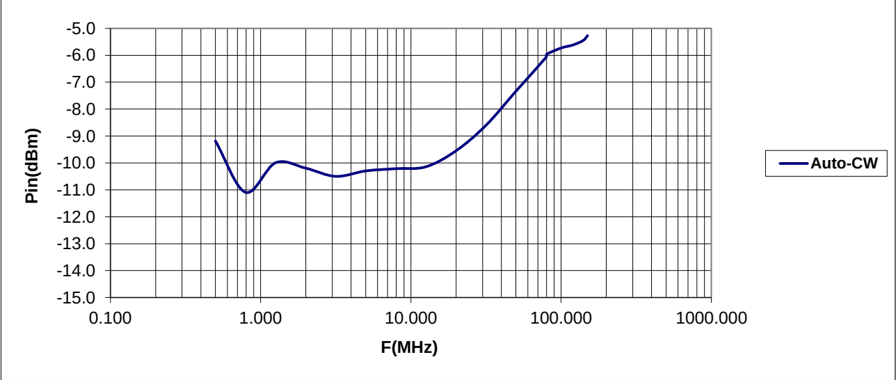
Input Power (dBm) for 50W Out in CW mode
