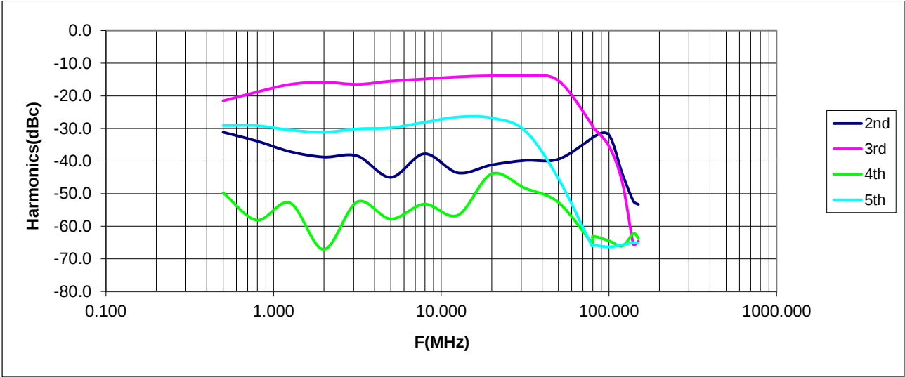
Harmonics Measured @ Pout = P1dB spec.
