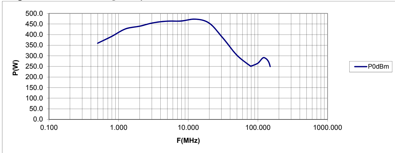
P1dB Measured @10% Duty, 100uS Pulse Width
