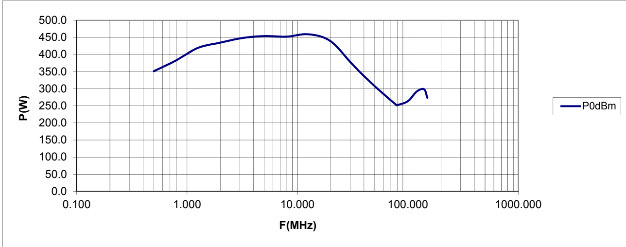
P1dB Measured @10% Duty, 100uS Pulse Width
