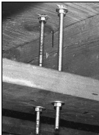
Fig 46 —The strengthened anchoring for the tripod. Bolts are placed through two 2 × 6s on the underside of the roof and through the 2 × 6 on the top of the roof, as shown in Fig 43.
