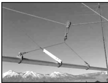
Fig 36—Photo of the tram system used by Kurt Address, K7NV. (Photo by K7NV.)
