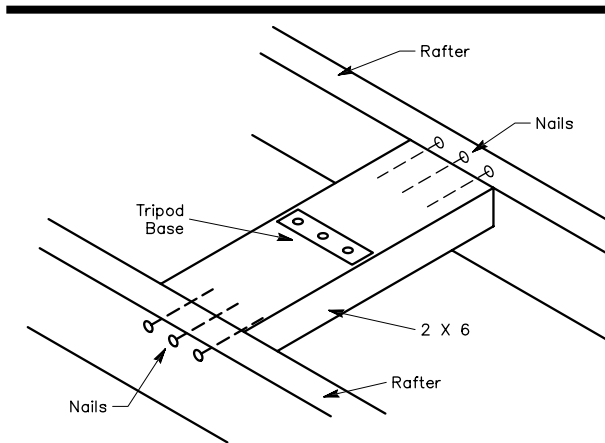
Fig 44 —This cutaway view illustrates how the tripod tower is secured to the roof rafters. The leg to be secured to the crosspiece is placed on the outside of the roof. Another cross member is fastened to the underside of the rafters. Bolts, inserted through the roof and the two cross pieces, hold the inner cross member in place because of pressure applied. The inner crosspiece can be nailed to the rafter for added strength.
