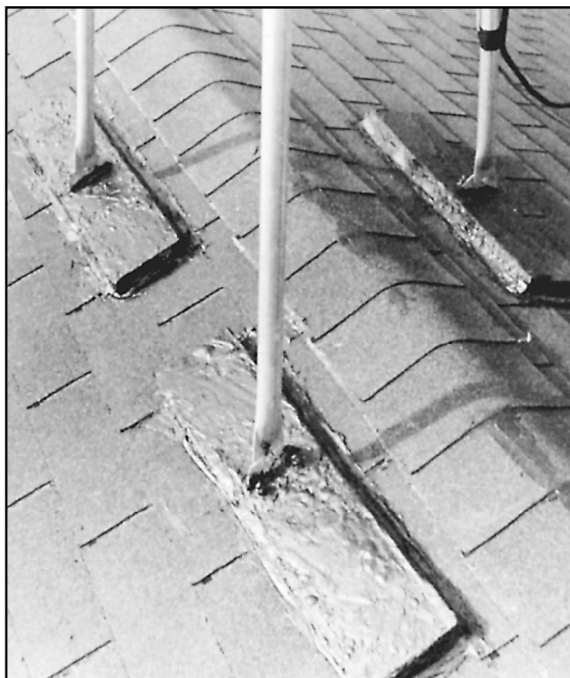
Fig 45 —Three lengths of 2 × 6 wood mounted on the outside of the roof and reinforced under the roof by three identical lengths provide a durable means for anchoring the tripod. A thick coat of roofing tar guards against weathering and leaks.
