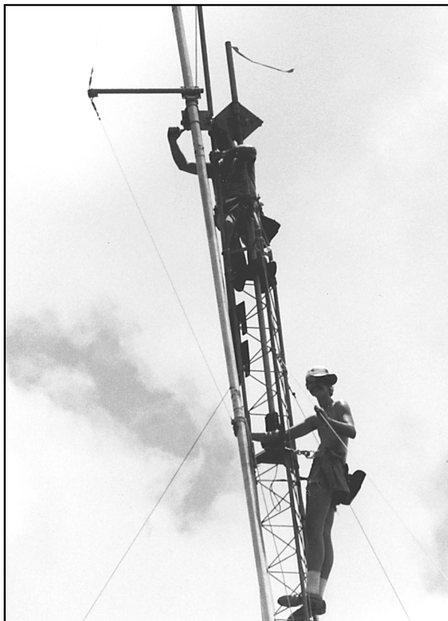
Fig 40—Working at the 70-foot level. A gin pole makes pulling up and mounting the boom to the boom plate a safe and easy procedure.
