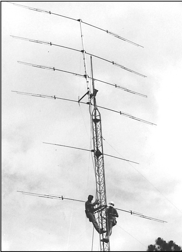
Fig 41—Mounting the last element prior to positioning the boom in a horizontal plane.
