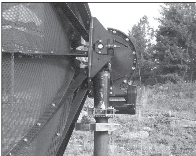
Fig 67 —A modified TVRO dish mount is shown using an Az-EI mount and a sector-gear drive for the elevation. (W0LMD photo.)
