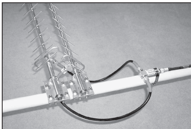
Fig 14—An example of offset crossed-Yagi circularly polarized antennas with fixed polarization. This example is a pair of M² 23CM22EZA antennas, for L band (1269 MHz), mounted on an elevation boom. (WD4FAB photo.)
