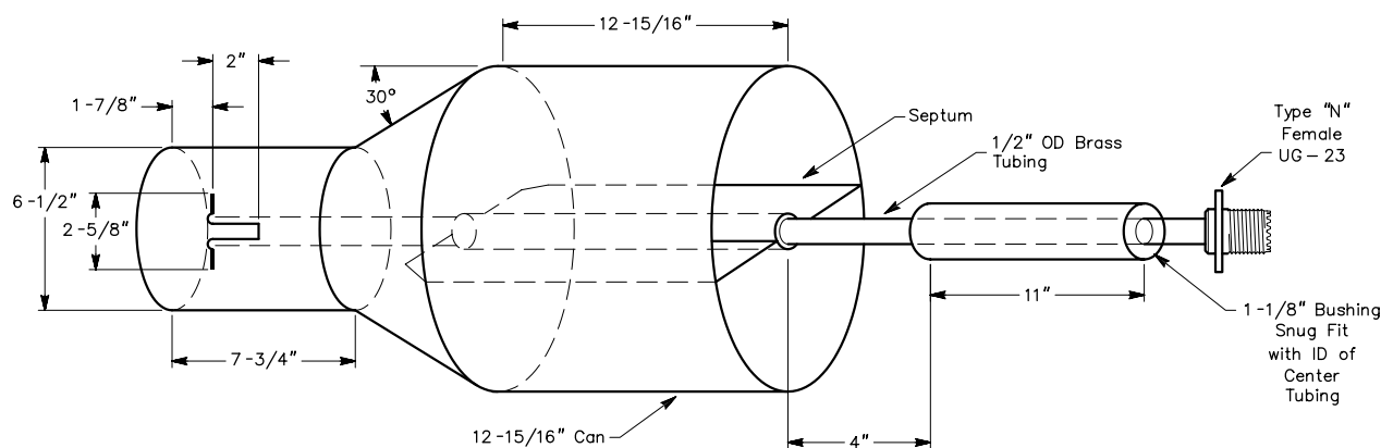
Fig 82—Backfire type 1296-MHz feed horn, linear polarization only. The small can is a Quaker State oil container; the large can is a 50-pound shortening container (obtained from a restaurant, Gold Crisp brand). Brass tubing, 1/2-inch OD extends from UG-23 connector to dipole. Center conductor and dielectric are obtained from 3/8-inch Alumaflex coaxial cable. The dipole is made from 3/32-inch copper rod. The septum and 30° section are made from galvanized sheet metal. Styrofoam is used to hold the septum in position. The primary gain is 12.2 dBi.
