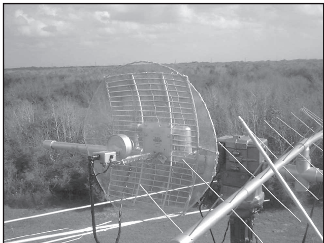
Fig 28 —K5GNA's "circularized" mesh modification of an MMDS dish antenna with a helix-CP feed and DEP preamp. The dish modification reduces the spillover loss by making the antenna fully circular. ( K5OE photo. )
