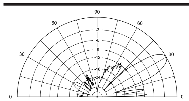
Fig 72—EZNEC Pro elevation pattern for four 14-element 2-meter Yagis ( 3.6\lambda boom lengths) at an elevation angle of 30° above the horizon. The computed system gain is 21.5 dBi, suitable for 2-meter EME. This assumes that the phasing system is made of open-wire transmission lines so that feed-line losses can be kept below 0.25 dB.
