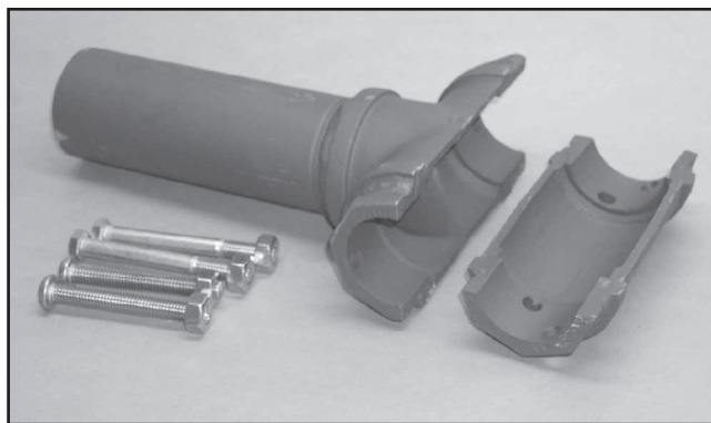
Fig 46—Welded pipefitting mount bracket for FABStar dish antenna. (WD4FAB photo.)
