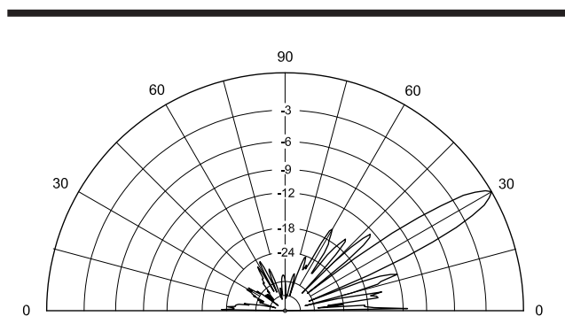
Fig 74—Computed elevation response for K1FO 16-Yagi 432-MHz array shown in Fig 73. (The EZNEC Pro model required 2464 segments!) With assumed phasing harness feed-line losses of 0.25 dB, the overall gain exceeds 27.5 dBi.
