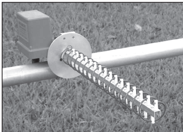
Fig 36 —WD4FAB's example of a 16-turn S-band helical antenna for AO-40. This is about the maximum length of any practical helix. Note the SSB UEK2000 downconverter mounted behind the reflector of the antenna. (WD4FAB photo.)
