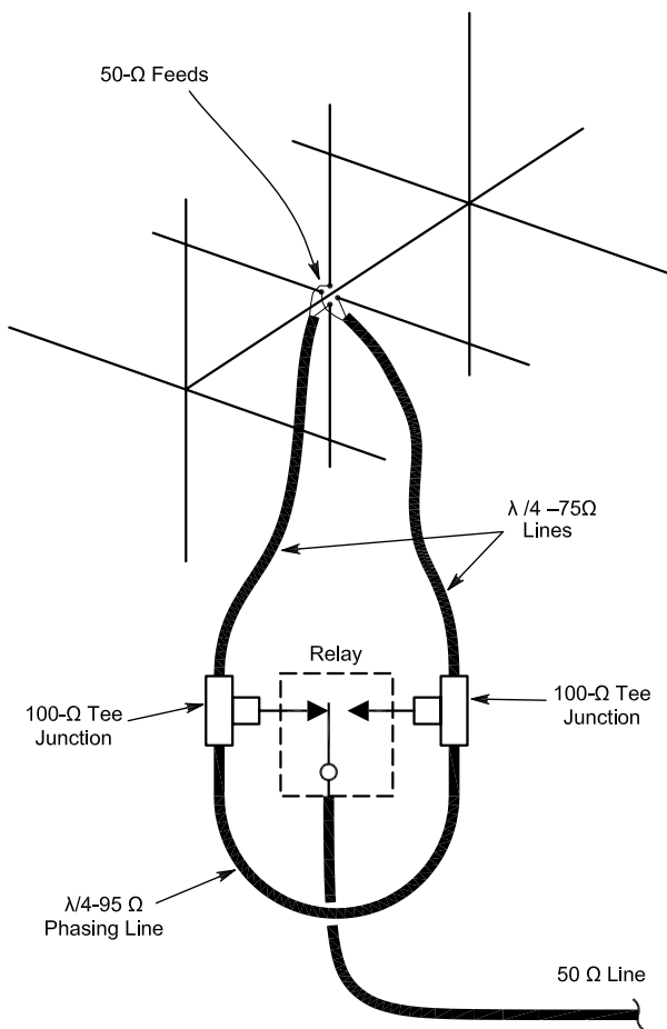
Fig 10—Co-planar crossed Yagi, circularly polarized antenna with switchable polarization phasing harness.
