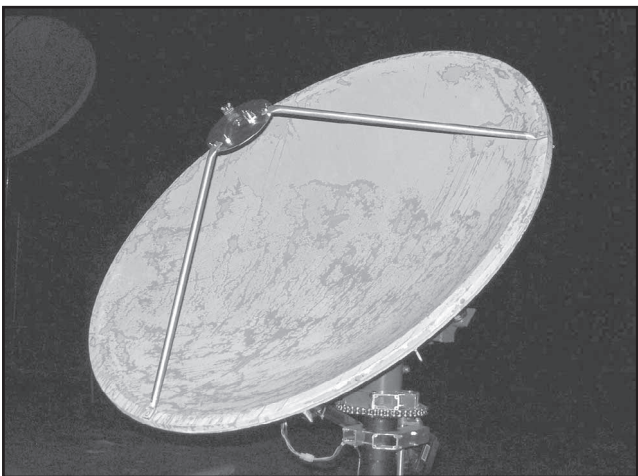
Fig 23 —Robert Suding, W0LMD, modified this 4-foot dish antenna with a patch feed for S band and an Az-EI mount. (W0LMD photo.)
