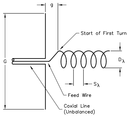
Fig 16—The basic helical antenna and design equations.
