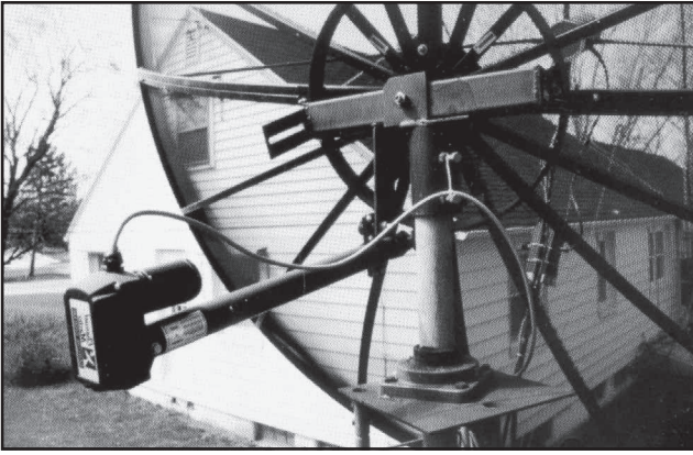
Fig 90—Elevation system, showing modified TVRO mount.
