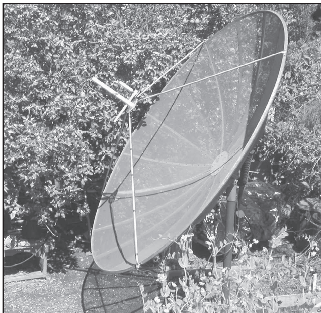
Fig 27 —Clair E. Cessna, K6LG, has this 10-foot dish with S-band patch feed. This dish uses the original polar-mounting system and offsets the patch feed to compensate for AO-40's deviation from the Clarke belt. ( K6LG photo. )
