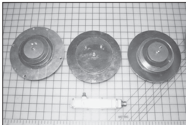
Fig 49—Some of the many experimental CP-patch-feed antennas by W0LMD. (W0LMD photo.)
