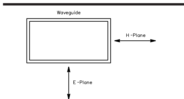
Fig 74 —10-GHz antennas are usually fed with waveguide. See text for a discussion of waveguide propagation characteristics.
