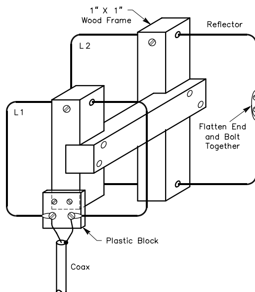
Fig 55—Mechanical details of a 2-element quad for 144 MHz. The driven element, L1, is one wavelength long; reflector L2 is 5% longer. With the transmission line connected as shown here, the resulting radiation is horizontally polarized. Sets of elements of this type can be stacked horizontally and vertically for high gain with broad frequency response. Recommended bay spacing is \frac{1}{2} \lambda between adjacent element sides. The example shown may be fed directly with 50- \Omega coax.
