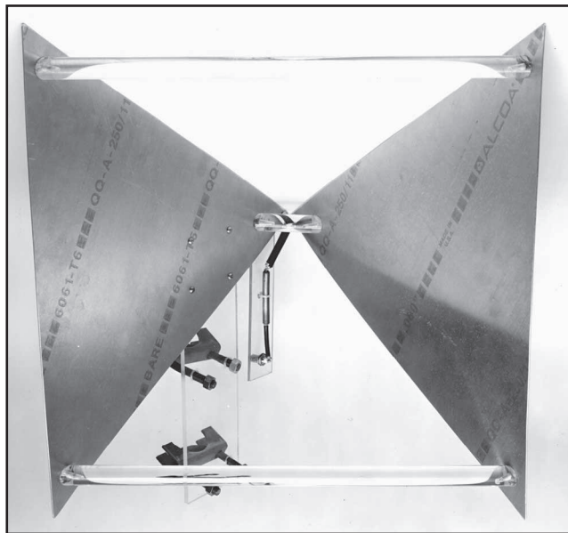
Fig 22 —An experimental two-sided pyramidal horn constructed in the ARRL laboratory. A pair of muffer clamps allows mounting the antenna on a mast. This model has sheet-aluminum sides, although window screen would work as well. Temporary elements could be made from cardboard covered with aluminum foil. The horizontal spreaders are Plexiglas rod. Oriented as shown here, the antenna radiates horizontally polarized waves.
