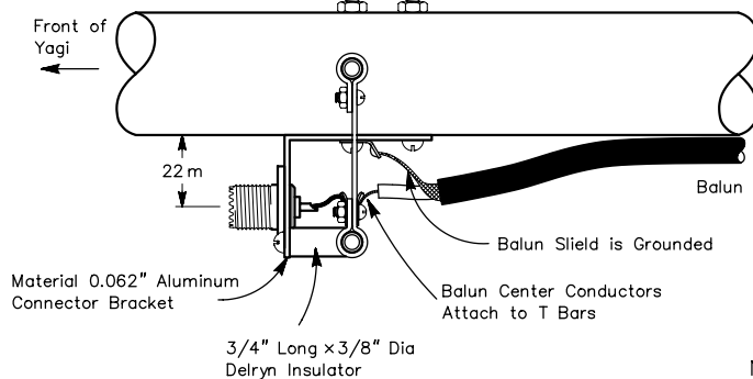
Driven Element Side View
