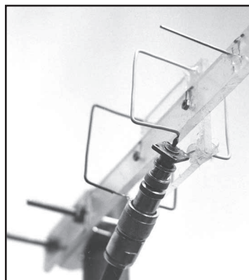
Fig 66 —A view of the 10-element version of the 1296-MHz Quagi. It is mounted on a 30-in. Plexiglas boom with a 3 x 3-in. square of Plexiglas to support the driven element and reflector. Note how the driven element is attached to a standard UG-290 BNC connector. The elements are held in place with silicone sealing compound.
