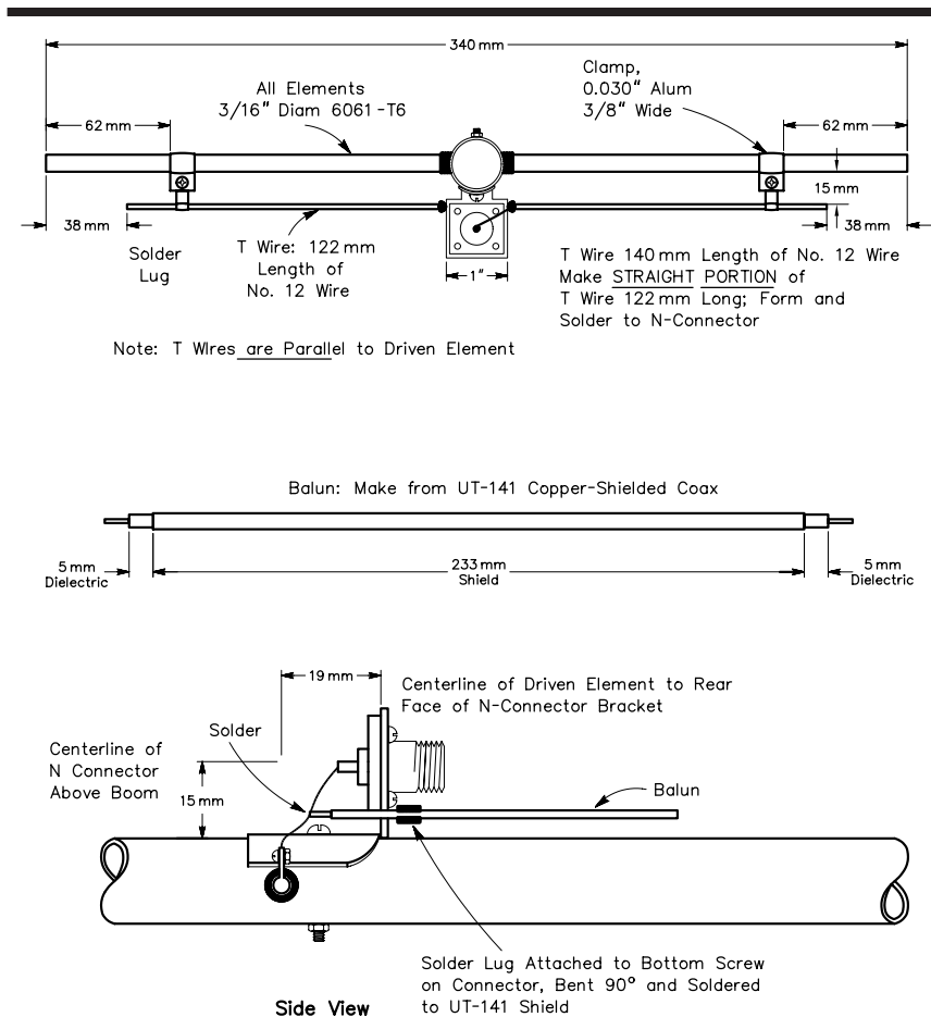
Fig 44—Details of the driven element and T match for the 22-element Yagi. Lengths are given in millimeters to allow precise duplication of the antenna. See text.
