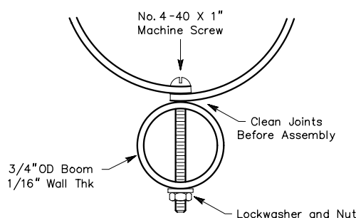
Fig 71—Element-to-boom mounting details.
