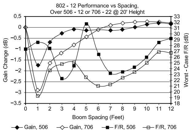
Fig 11 —Plot of 8-element 2-meter Yagi's gain and worst-case F/R as a function of distance over two types of 6-meter beams, one on a 12-foot boom and the other on a 22-foot boom. Beyond a spacing of about 5 feet the performance is degraded a minimal amount.
