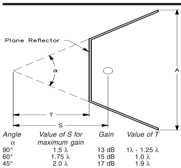
Fig 21—The trough reflector. This is a useful modification of the corner reflector. The vertex has been cut off and replaced by a simple plane section. The tabulated data shows the gain obtainable for greater values of S than those covered in Table 2, assuming that the reflector is of adequate size.
