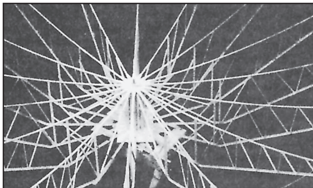
Fig 29 —Detailed look at the hub assembly for the ZL1BJQ dish. Most of the structural members are made from 3/4-inch T section.
