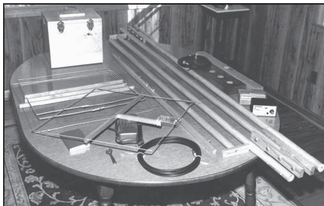
Fig 57—The complete portable quad, broken down for travel. Visible in the foreground is the driven element. The pine box in the background is a carrying case for equipment and accessories. A hole in the lid accepts the mast, so the box doubles as a base for a short mast during portable operation. (W1MPO photo)
