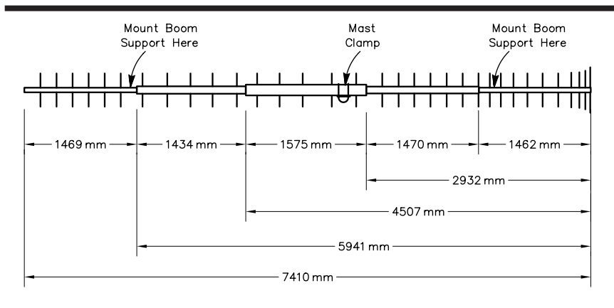
Fig 46—Boom-construction information for the 33-element Yagi. Lengths are given in millimeters to allow precise duplication of the antenna.
