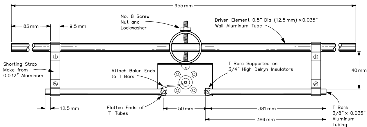
Driven Element Detail 12-Element 144 MHz Yagi
