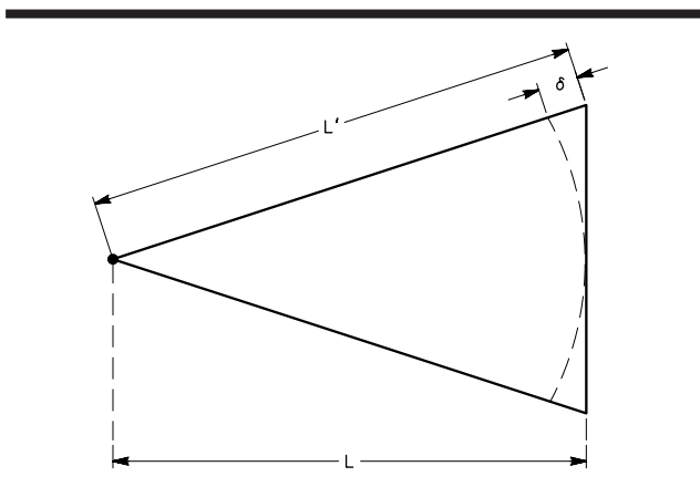
Fig 75 —The path-length (phase) difference between the center and edge of a horn antenna is \delta .
