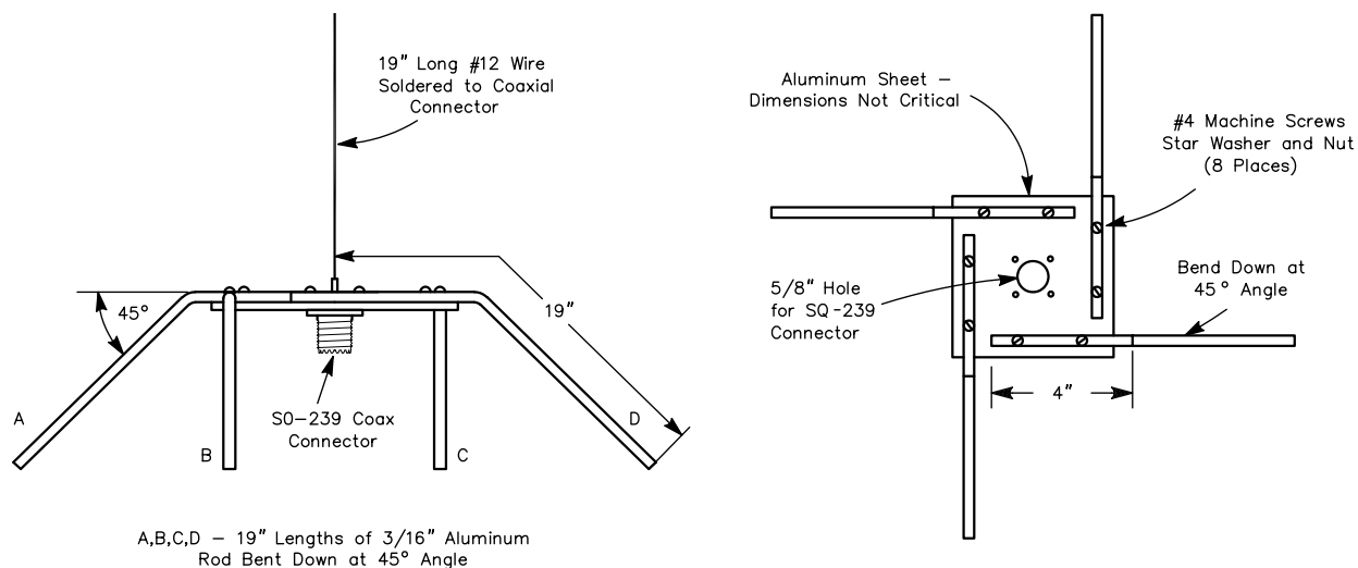
Fig 30— These drawings illustrate the dimensions for the 144-MHz ground-plane antenna. The radials are bent down at a 45° angle.
