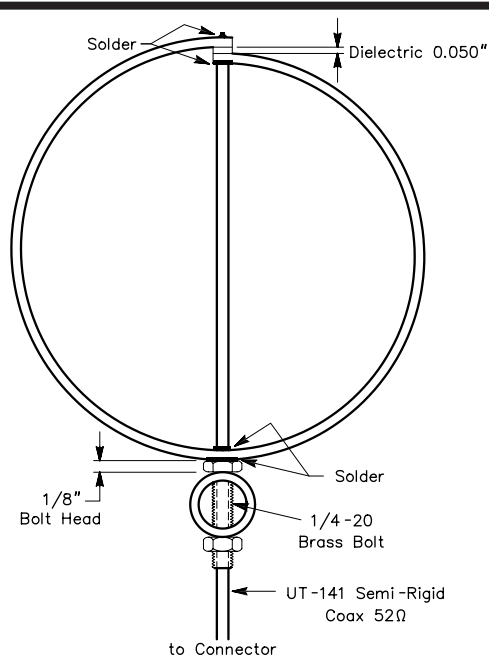
Fig 72—Driven-element details. See Fig 70 and the text for additional information.
