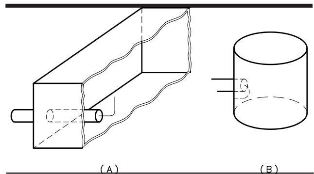
Fig 2—Coupling coaxial line to waveguide and resonators.
