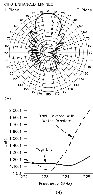
Fig 54—H- and E-plane patterns for the 16-element 222-MHz Yagi at A. The driven-element T-match dimensions were chosen for the best SWR compromise between wet and dry weather conditions. The SWR vs frequency curve shown at B demonstrates the broad frequency response of the Yagi design.
