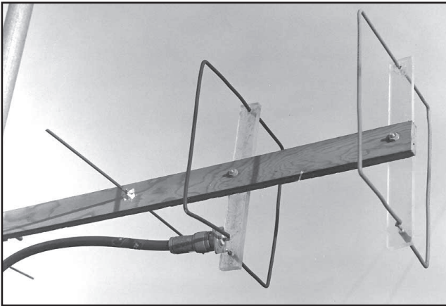
Fig 65 —A close-up view of the feed method used on a 432-MHz Quagi. This arrangement produces a low SWR and gain in excess of 13 dBi with a 4-ft 10-in. boom! The same basic arrangement is used on lower frequencies, but wood may be substituted for the Plexiglas spreaders. The boom is 1/2-in. exterior plywood.
