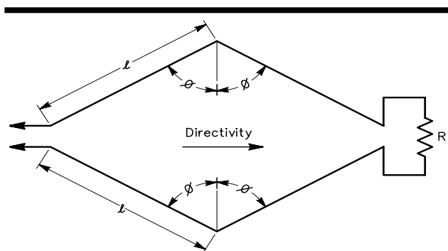
Fig 24—The layout for a terminated rhombic antenna.
