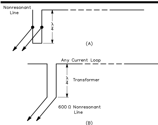
Fig 8—Methods for feeding long single-wire antennas.
