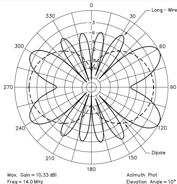
Fig 4—An azimuthal-plane comparison between a 3\text{-}\lambda (209 feet long) long-wire (solid line) and the comparison \frac{1}{2}\text{-}\lambda dipole (dashed line) at 70 feet high ( 1\lambda ) at 14 MHz.
