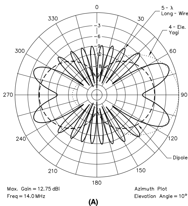
Fig 6—At A, the azimuth responses for a 5- \lambda long-wire (350 feet long at 14 MHz—solid line) to the same 4-element Yagi (dotted line) and dipole (dashed line) as in Fig 5. At B, the elevation-plane responses for the long-wire (solid line) and the dipole (dashed line) by themselves. Note that the elevation angle giving peak gain for each antenna is just about the same. The long-wire achieves gain by compressing mainly the azimuthal response, squeezing the gain into narrow lobes; not so much by squeezing the elevation pattern for gain.
