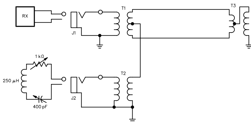
Fig 37—A two-wire Beverage antenna that has provisions for direction switching and null steering in the rear quadrant. Performance improves with height to a point, and is optimum for 1.8-MHz operation at about 10 to 12 feet. Parts identifications are for text reference.
