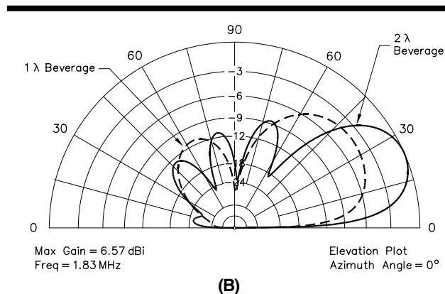
Fig 35—At A, azimuthal patterns of a 2-λ (solid line) and a 1-λ (dashed line) Beverage antenna, terminated with 550-Ω resistor at 1.83 MHz, at an elevation angle of 10°. The rearward pattern around 180° is more than 20 dB down from the front lobe for each antenna. At B, the elevation-plane patterns. Note the rejection of very high-angle signals near 90°.
