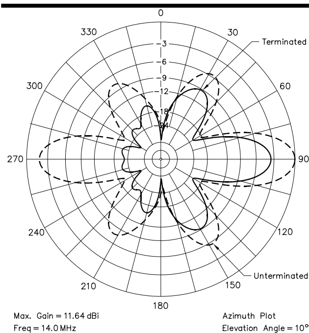
Fig 23—The azimuthal patterns for a shorter-leg V-beam (2- \lambda legs) when it is terminated (solid line) and unterminated (dashed line). With shorter legs, the terminated V-beam loses about 3.5 dB in forward gain compared to the unterminated version, while suppressing the rearward lobes as much as 20 dB.
