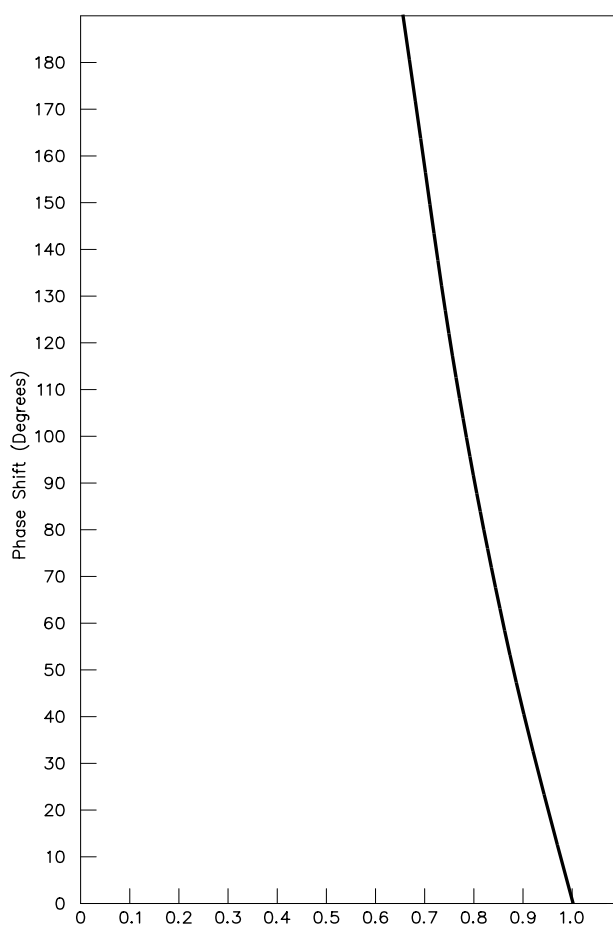
Fig 33—This curve shows phase shift (per wavelength) as a function of velocity factor on a Beverage antenna. Once the phase shift for the antenna goes beyond 90^\circ , the gain drops off from its peak value, and any increase in antenna length will decrease gain.
