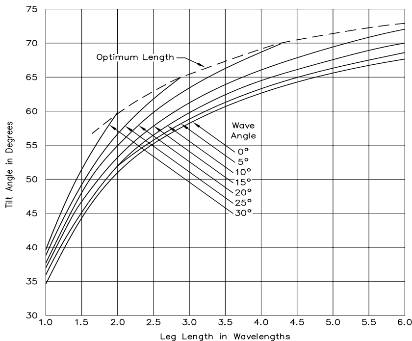
Fig 25—Rhombic-antenna design chart. For any given leg length, the curves show the proper tilt angle to give maximum radiation at the selected takeoff angle. The broken curve marked “optimum length” shows the leg length that gives the maximum possible output at the selected takeoff angle. The optimum length as given by the curves should be multiplied by 0.74 to obtain the leg length for which the takeoff angle and main lobe are aligned.
