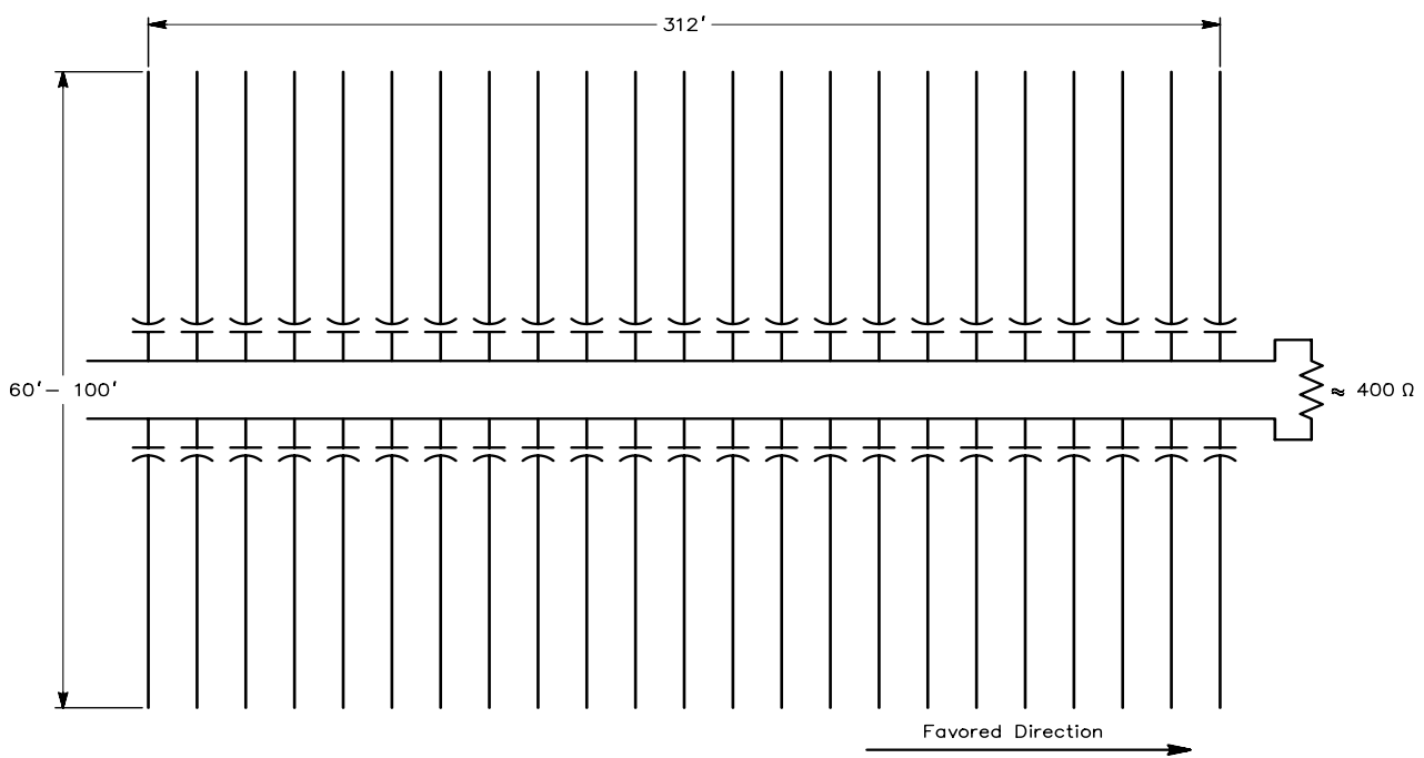
Fig 39—The fishbone antenna provides higher gain per acre than does a rhombic. It is essentially a wave antenna that evolved from the Beverage.
