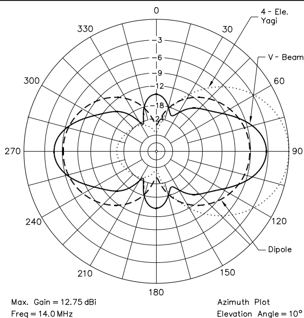
Fig 10— Azimuthal-plane pattern at 10° elevation angle for a 14-MHz V-beam (solid line) with 1- \lambda legs (68.5 feet long), using an included angle of 75° between the legs. The V-beam is mounted 1 \lambda above flat ground, and is compared with a \frac{1}{2} - \lambda dipole (dashed line) and a 4-element 20-meter Yagi on a 26-foot boom (dotted line).
