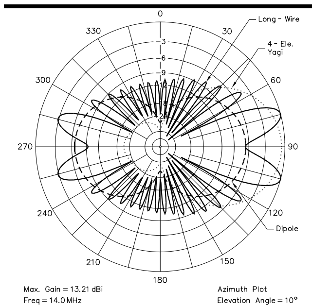
Fig 7—The azimuthal-plane performance for an 8- \lambda (571 feet) long-wire antenna (solid line), compared with a 4-element Yagi (dotted line) and a \frac{1}{2} - \lambda dipole (dashed line).
