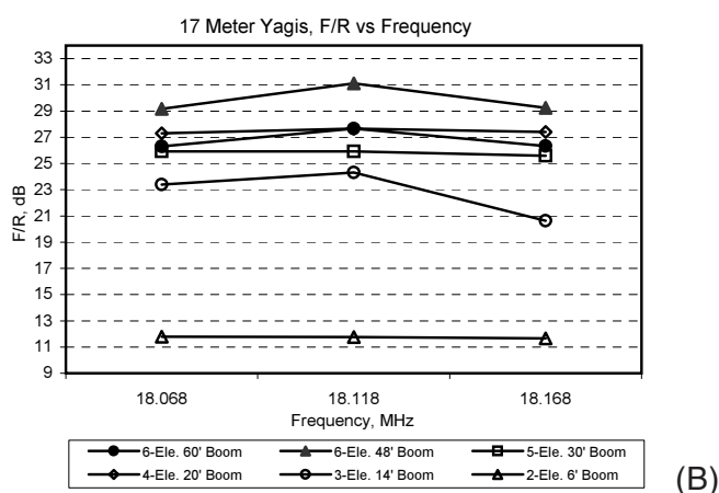
Fig 16—Gain, F/R and SWR performance versus frequency for optimized 17-meter Yagis. At A, gain versus frequency is shown for six 17-meter Yagis whose booms range from 6 feet to 60 feet long. Except for the 2-element design, these Yagis have been optimized for better than 20 dB F/R and less than 2:1 SWR over the narrow 17-meter band 18.068 to 18.168 MHz. At B, front-to-rear ratio for these antennas is shown versus frequency, and at C, SWR over the frequency range is shown. At D, the taper schedule for heavy-duty and for medium-duty 10-meter elements is shown. The heavy-duty elements can withstand 123-mph winds without icing, and 89-mph winds with \frac{1}{4} -inch radial ice. The medium-duty elements can survive 83-mph winds without icing, and 59-mph winds with \frac{1}{4} -inch radial ice. The wall thickness for each telescoping section of 6061-T6 aluminum tubing is 0.058 inches, and the overlap at each telescoping junction is 3 inches.
