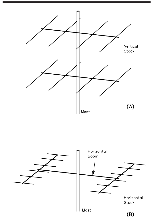
Fig 26—Stacking arrangements. At A, two Yagis are stacked vertically (broadside) on the same mast. At B, two Yagis are stacked horizontally (collinear) side-by-side. At HF the vertical stack is more common because of mechanical difficulties involved with large HF antennas stacked side-by-side, whereas at VHF and UHF the horizontal stack is common.
