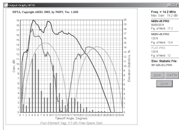
Fig 47— HFTA screen shot showing how complicated things become when real-world irregular terrain is analyzed. This is the 20-meter elevation pattern for the N6BV/1 station location in Windham, NH, for the 90/60/30-foot stack of triband TH7DX Yagis and a 4-element Yagi at 120 feet on the same tower. For comparison, the response of a 120-foot Yagi over flat ground is also included.
