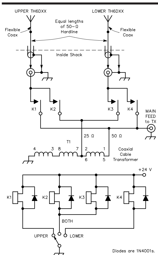
Fig 40—Relay switch box for K1VR stacked tribander system. Equal lengths of 50-Ω Hardline (with equal lengths of flexible 50-Ω cable at each antenna to allow rotation) go to the switch box in the shack. The SWR on all three bands for Upper, Lower or Both switch positions is very close to constant.
