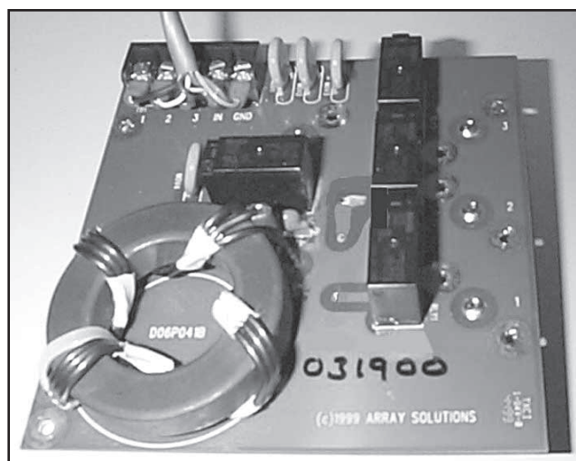
Fig 43—Inside view of StackMatch. (Photo courtesy Array Solutions.)
