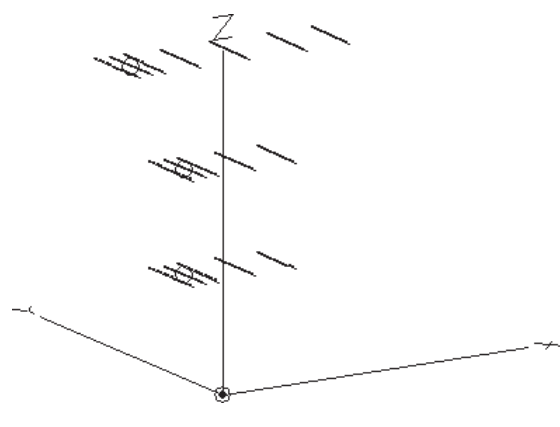
Fig 45—Stacking dissimilar Yagis. In this case a 7-element 10-meter Yagi is stacked over two 5-element Yagis. Note the displacement of the 7-element Yagi’s driven element compared to the position of the two 5-element Yagis. This leads to an undesired phase shift for the higher antenna.
