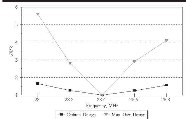
Fig 4—SWR over the 28.0 to 28.8 MHz portion of the 10-meter band for two different 3-element Yagi designs. One is designed strictly for maximum gain, while the second is optimized for F/R pattern and SWR over the frequency band. A Yagi designed only for maximum gain usually suffers from a very narrow SWR bandwidth.
