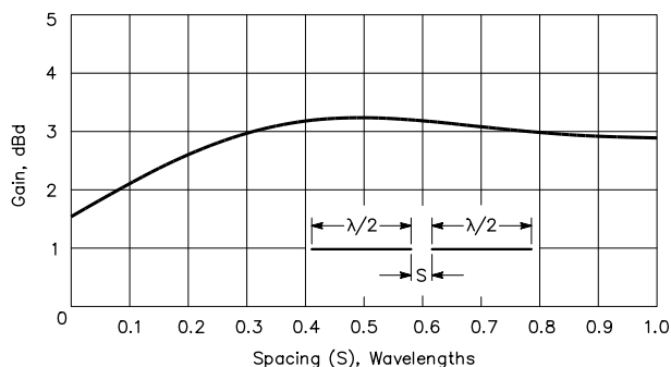
Fig 39—Gain of two collinear 1/2\text{-}\lambda elements as a function of spacing between the adjacent ends.
