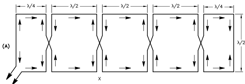
Fig 46 —Typical Sterba array, an 8-element version.
