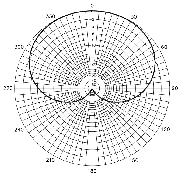
Fig 69—H-plane pattern for a 3-element end-fire array with binomial current distribution (the current in the center element is twice that in each end element). The elements are spaced \frac{1}{4} \lambda apart along the 0°-180° axis. The center element lags the lower element by 90°, while the upper element lags the lower element by 180° in phase. Dissimilar current distributions are taken into account. (Pattern computed with ELNEC .)
