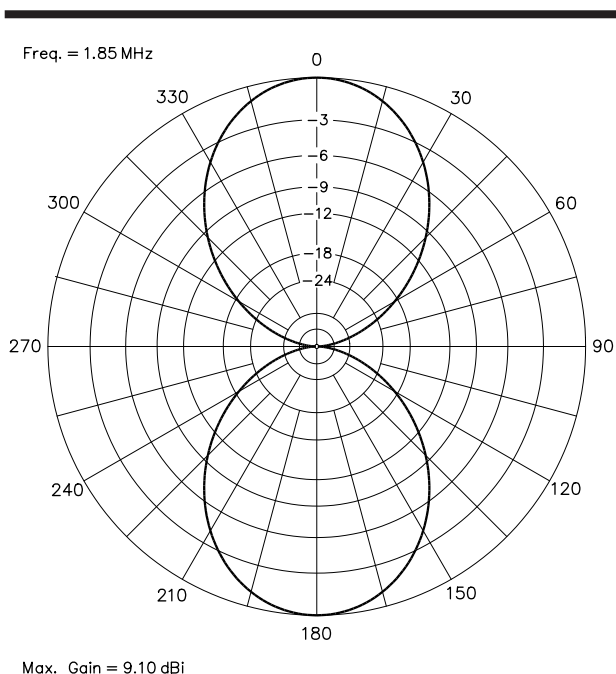
Fig 78—Free-space H-plane pattern of the four-element antenna shown in Fig 77.
