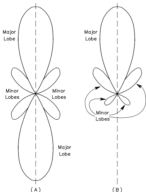
Fig 5 —At A, typical bidirectional pattern and at B, unidirectional directive pattern. These drawings also illustrate the application of the terms major and minor to the pattern lobes.
