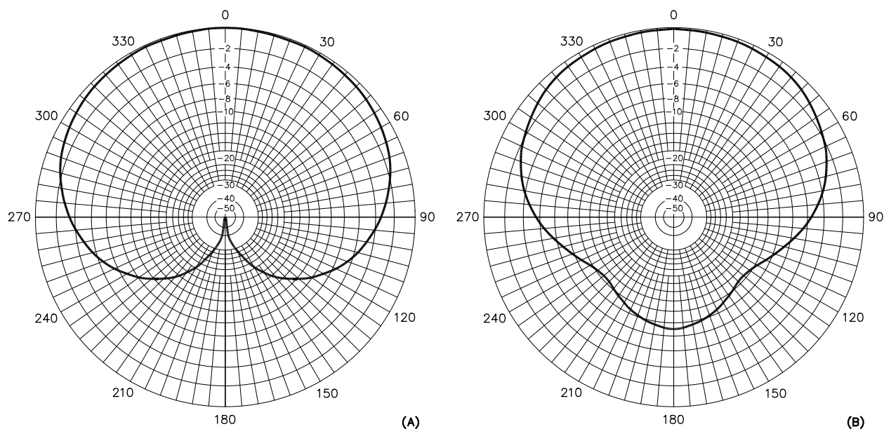
Fig 23—Patterns of an array when correctly fed, A, and when casually fed, B. (See text. Similar current distributions are assumed.) The difference in gain is about 0.1 dB. Gain is referenced to a single similar element; add 3.1 dB to the scale values shown.
