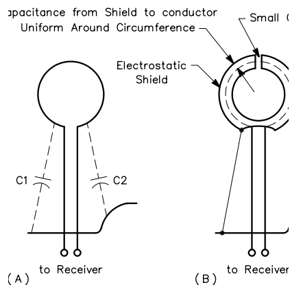
Fig 8—At A, the loop is unbalanced by capacitance to its surroundings. At B, the use of an electrostatic shield overcomes this effect.
