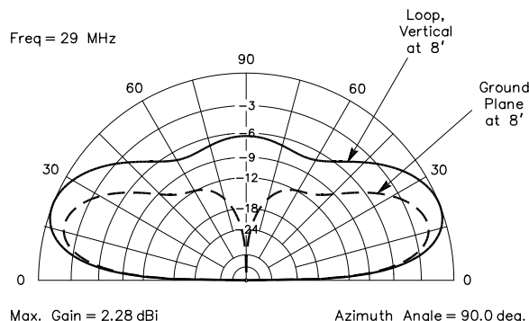
Fig 20—Elevation-plane plot for a 16.2-inch wingspan octagonal copper loop at 29 MHz, compared to a \lambda/4 ground-plane antenna with two resonant elevated radials. The gains at low angles are almost identical, but the loop exhibits more gain at medium and high elevation angles. Again, the bottom of each antenna is located 8 feet above ground for safety.
