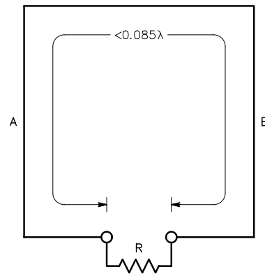
Fig 5—Simple untuned small loop antenna.
