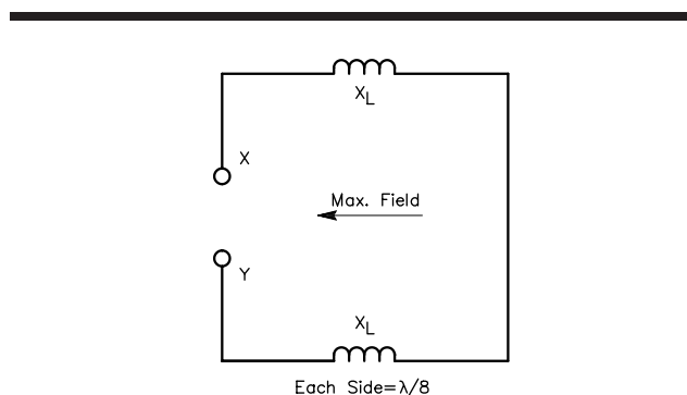
Fig 2—Inductive loading in the sides of a \frac{1}{2} \lambda loop to increase the directivity and gain. Maximum radiation or response is in the plane of the loop, in the direction shown by the arrow.
