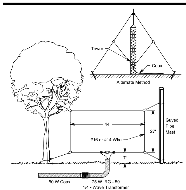
Fig 30—At A, details of the rectangular full-wave loop. The dimensions given are for operation at 7.05 MHz. The height above ground was 7 feet in this instance, although improved performance should result if the builder can install the loop higher above ground without sacrificing length on the vertical sides. At B, illustration how a single supporting structure can be used to hold the loop in a diamond-shaped configuration. Feeding the diamond at the lower tip provides radiation in the horizontal plane. Feeding the system at either side will result in vertical polarization of the radiated signal.
