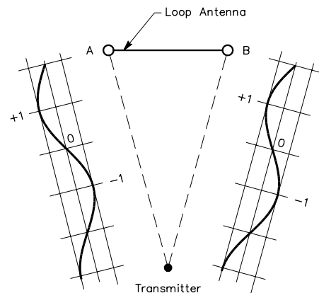
Fig 6—Example of orientation of loop antenna that does not respond to a signal source (null in pattern).
