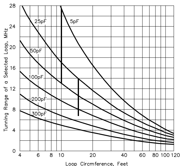
Fig 19—Frequency tuning range of an octagon-shaped loop using \frac{3}{4} -inch copper water pipe, for various values of tuning capacitance and loop circumference.
