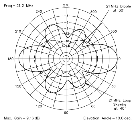
Fig 27 —At A, azimuth-plane response of 142-foot long, 7-MHz Loop Skywire, 40 feet in the air at 7.2 MHz, compared with \frac{1}{2}\lambda dipole 30 feet in the air. At B, response of same Loop Skywire at 14.2 MHz, compared with \frac{1}{2}\lambda 14.2-MHz dipole 30 feet in the air. Now the loop has some advantage in certain directions. At C, response of the same Loop Skywire at 21.2 MHz compared to a 21.2-MHz dipole at 30 feet. Here, the Loop Skywire has more gain in almost all directions than the simple dipole. All azimuth-plane patterns were made at 10° elevation.
