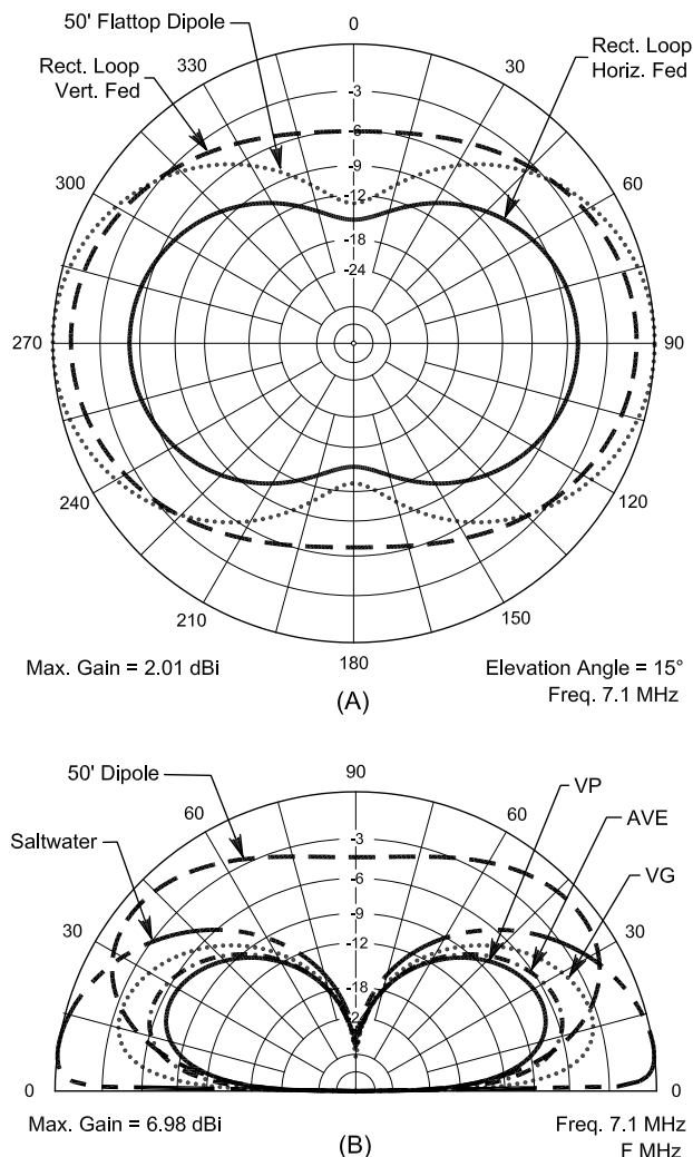
Fig 31—At A, azimuthal plane responses for the vertically and horizontally polarized 7-MHz loop, compared to a flattop 50-foot high dipole, all at a takeoff angle of 15° for DX work. The solid line is for feeding the loop horizontally at the bottom; the dashed line is for feeding the loop vertically at a side, and the dotted line is for a simple flattop horizontal dipole at 50 feet in height. For DX work, the vertically polarized loop is an excellent performer.
