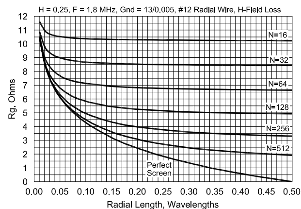
Fig 14—An example of the variation of R_g with radial length and number of radials ( N ) for h = 0.25 \lambda . When only a few radials are used there is little point in making them longer than 0.1 \lambda . Increasing N reduces R_g at a given radius and also makes longer radials useful, further reducing R_g . R_g for other values of h behave similarly.
