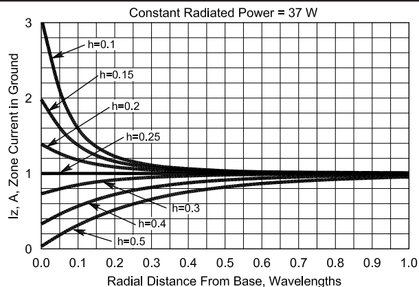
Fig 7—Plot of zone current ( I_z ) in amperes near the base of a vertical as a function of height ( h ) and radius ( r ) in wavelengths. The current in the base of the 0.25- \lambda antenna is assumed to be 1 A and the current for other values of h is adjusted to maintain the same radiated power ( P_r = I_o^2 R_r = 37 W) as the radiation resistance ( R_r ) changes with h .
