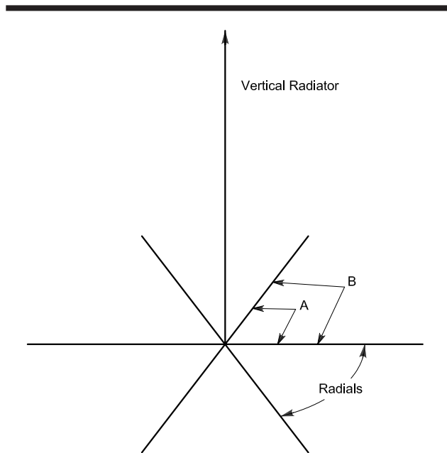
Fig 13—An example of current entering the ground between the radials and flowing for some distance before being picked up by a radial.
