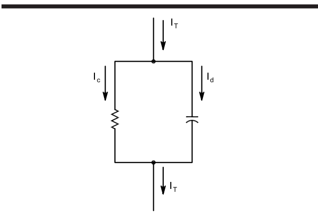
Fig 4— When the capacitor dielectric is less than perfect there will be a conduction current ( I_c ) in addition to the displacement current ( I_d ). Soil will typically have both resistive and capacitive components. Power loss in the soil is due to the current flowing through the resistive component.
