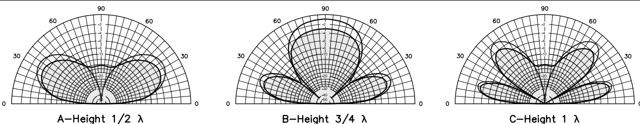
Fig 27—Vertical-plane radiation patterns of half-wave horizontal dipole antennas at 45^\circ from the antenna wire over flat ground. The solid-line and shaded curves represent the same conditions as in Figs 25 and 26. These patterns are scaled so they may be compared directly with those of Figs 25 and 26.
