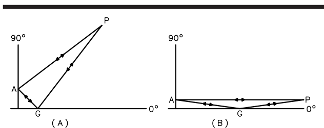
Fig 18—The direct wave and the reflected wave combine at point P to form the pattern (P is very far from the antenna). At A the two paths AP and AGP differ appreciably in length, while at B these two path lengths are nearly equal.
