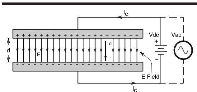
Fig 3— Example of an electric field, E=V_{dc}/d . When the dc source is replaced with an ac source there will be a displacement current ( I_d ) flowing between the capacitor plates.
