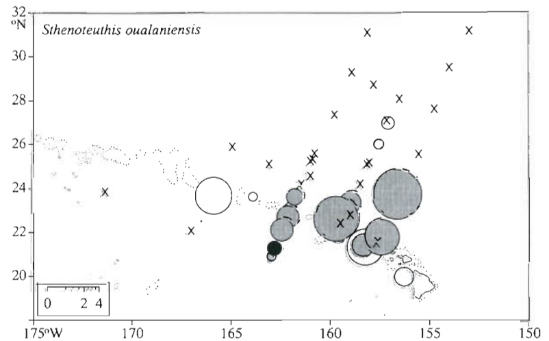
Fig. 2. Distribution and abundance of Sthenoteuthis oualaniensis . Symbols described in Fig. 1
