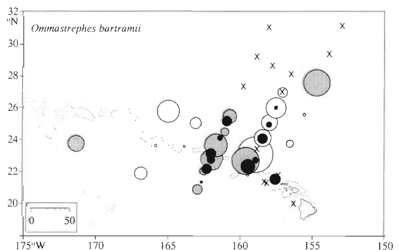
Fig. 1. Distribution and abundance of Ommastrephes bartramii paralarvae collected near the Hawaiian Islands during 5 cruises in 1991 to 1993. Circles represent mean station abundance (ind./50 m 2 ). White circles: 1991 catches; gray circles: 1992 catches; black circles: 1993 catches. Circle area represents catch abundance. X: no catch
