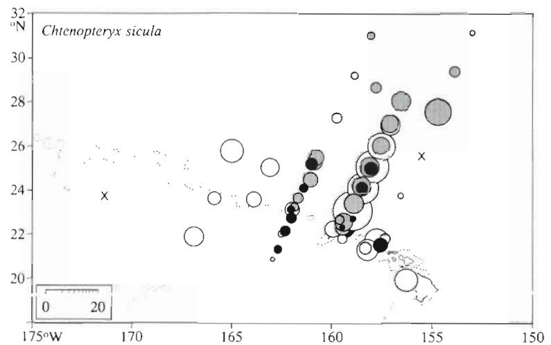
Fig. 8. Distribution and abundance of Ctenopteryx sicula . Symbols described in Fig. 1
